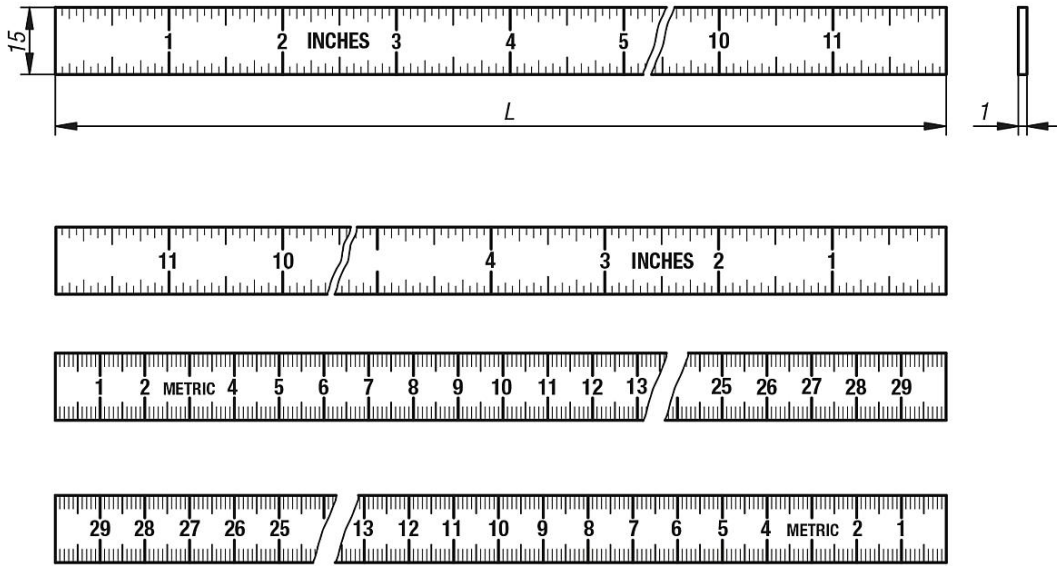
Vertical mounting
